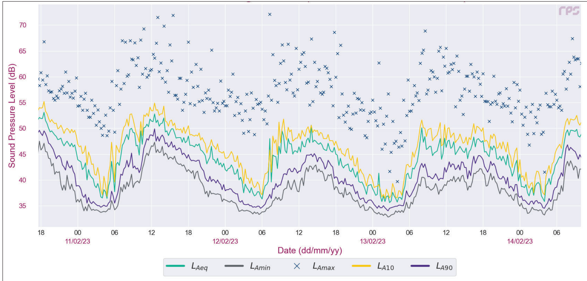
Figure 12.1.3: NML1 Complete Noise Data (10/02/2023 – 14/02/2023)
